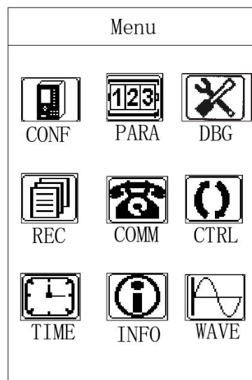
Figure 3.6 Main menu
