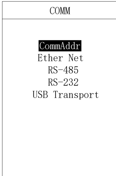
Fig. 3.19 Communication menu
